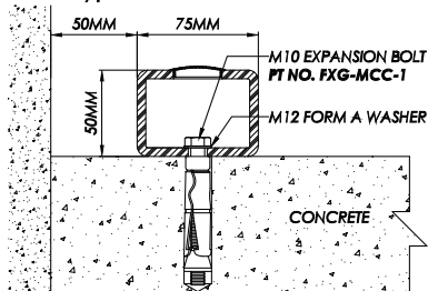
Typical Concrete Installations
