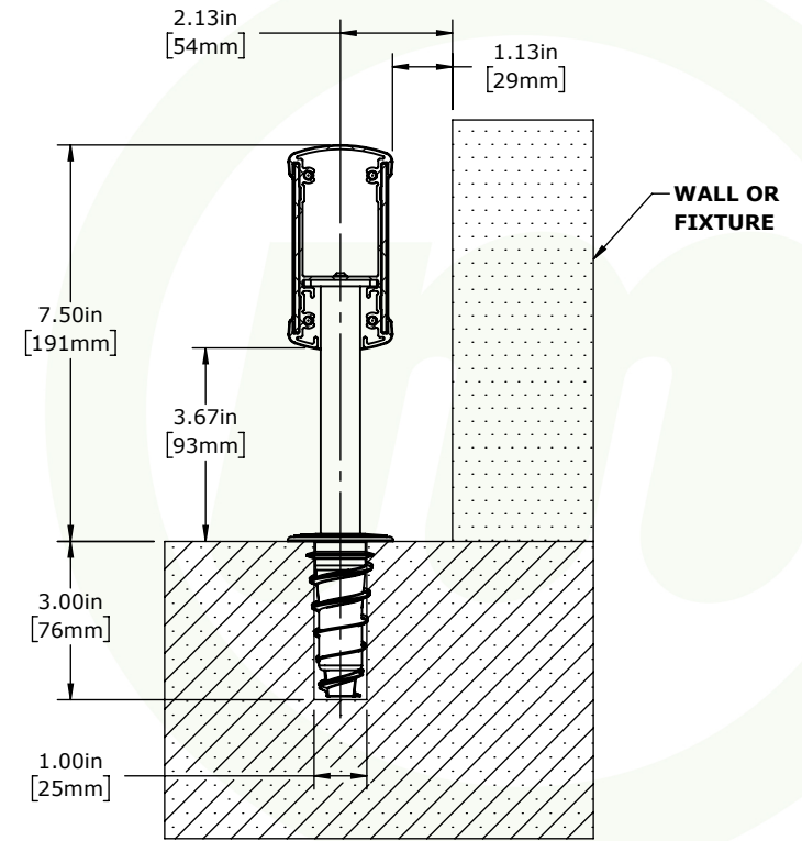
MOUNTING DETAIL
