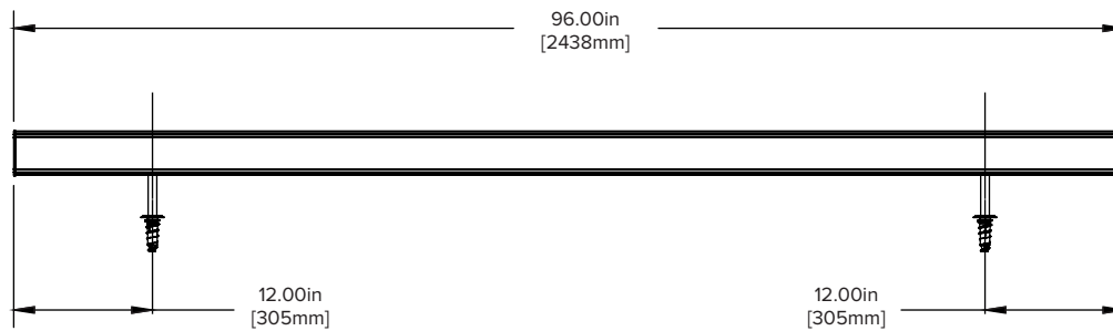
MOUNTING DETAIL
