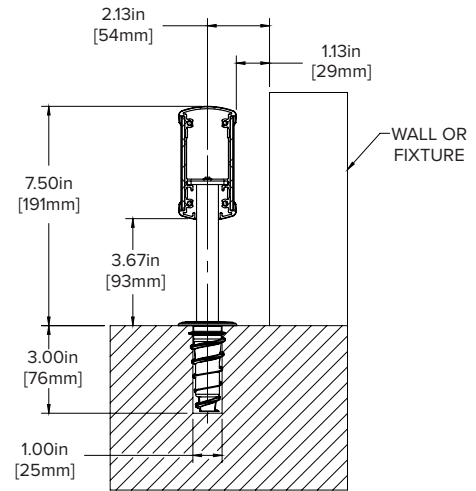
MOUNTING DETAIL
