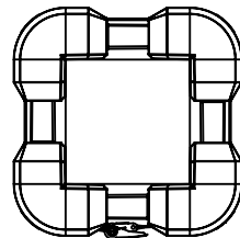
Top View Maximum Column Size 300mm x 300mm [12in x 12in]
