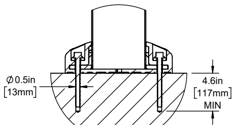
HOLE DETAIL SCALE 1 : 12
