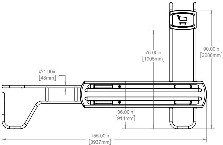
LEFT VIEW
