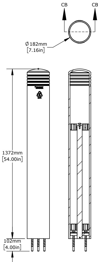
SECTION CB-CB
