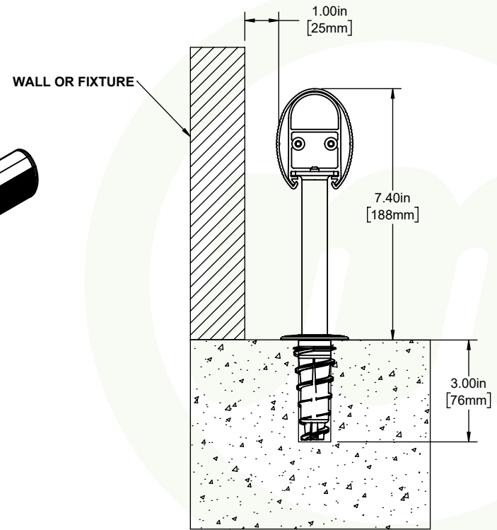
MOUNTING DETAIL
