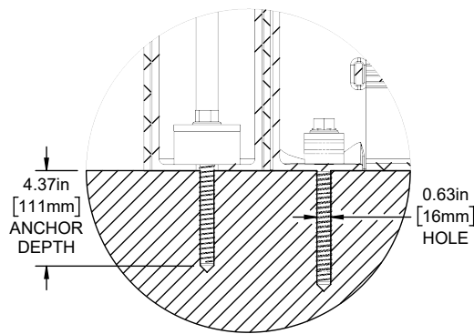
Fixing Detail
