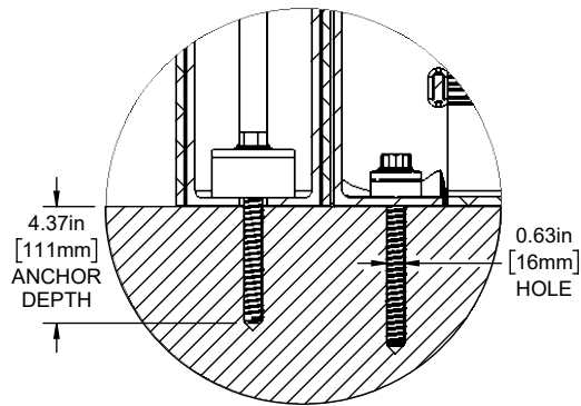
Fixing Detail
