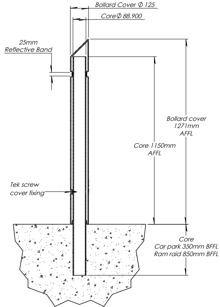
Bollard Specification
